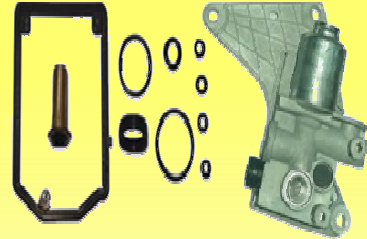
752 RPTO.VALV.EPG VOLVO 9700 20994250
