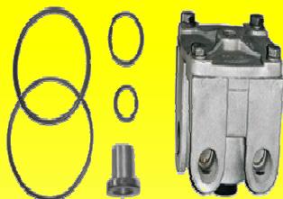
111 RPTO.VALVULA RELAY R-12
