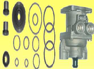
569 RPTO.P/VALV.PIE T/WABCO 008 0202 88450213
