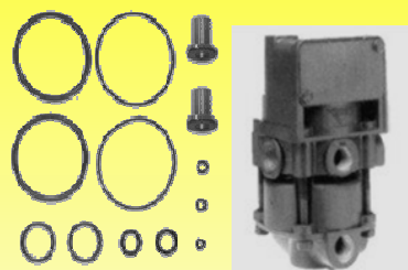
139 RPTO.VALV.WAGNER RS-2
