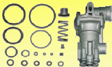
204 RPTO.VALV.RELEVO SEALCO 110200
